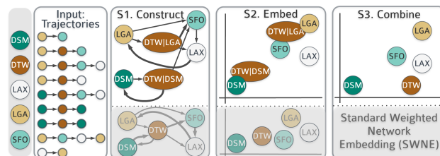
Figure 1: The proposed EVO framework (white background), contrasted with the standard approach SWNE (gray background) (§ IV-B). EVO takes trajectories as input (e.g., flight itineraries). Step 1 creates a HON that may contain multiple versions of a node (e.g., DTW is mapped to two conditional nodes (DTW|LGA & DTW|DSM) since the 0.5 probability of visiting SFO from DTW becomes 0.67 or 0.33 depending on how DTW was reached). Step 2 learns node embeddings from the HON. Step 3 combines the embeddings of all node versions into a single embedding capturing the important properties of all its versions. SWNE has only two steps.
